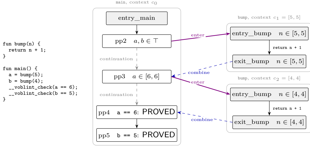
■ Figure 1 The running example. Left: the VIMP program. Right: its graph as the analyzer solves it with intervals and entry-state contexts. Each frame is one procedure in one context; bump gets one copy per entry state. Solid violet arrows are calls (enter), dashed blue arrows are returns (combine), and dashed gray arrows link a call site to its continuation. Both checks are PROVED . Without contexts, the single copy of bump joins both calls and both checks are UNKNOWN . The states shown are analyzer output using the warrowing update rule for global unknowns (Section 4). The drawing omits the intermediate node of bump 's body and the unreachable node after return .
