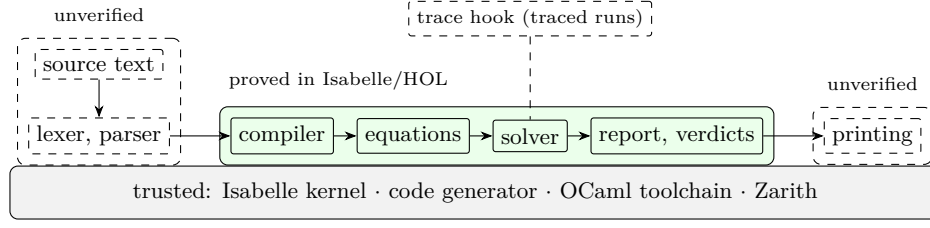
■ Figure 2 The trust boundary of the delivered analyzer, for programs for which the solver terminates. Dashed boxes are handwritten code outside the proof. For traced runs, the solver, routing functions, and report construction also call a trusted hook, which must return without exceptions and leave their results unchanged.
